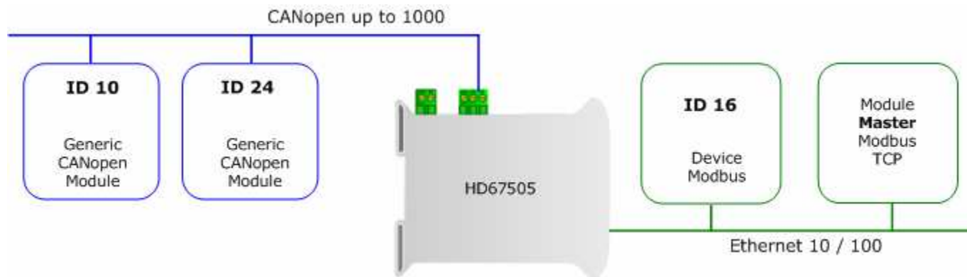
Figure 1: Connection scheme of HD67505 between a CANopen and Modbus TCP
