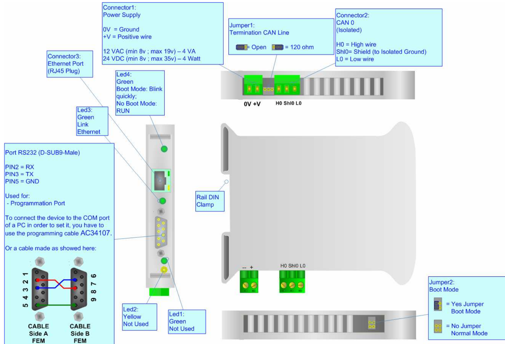
Figure 2: Connection Scheme for HD67505
