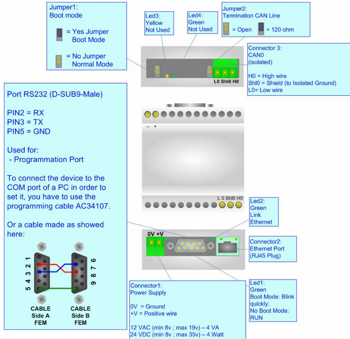
Figure 3: Connection Scheme for HD67505M
