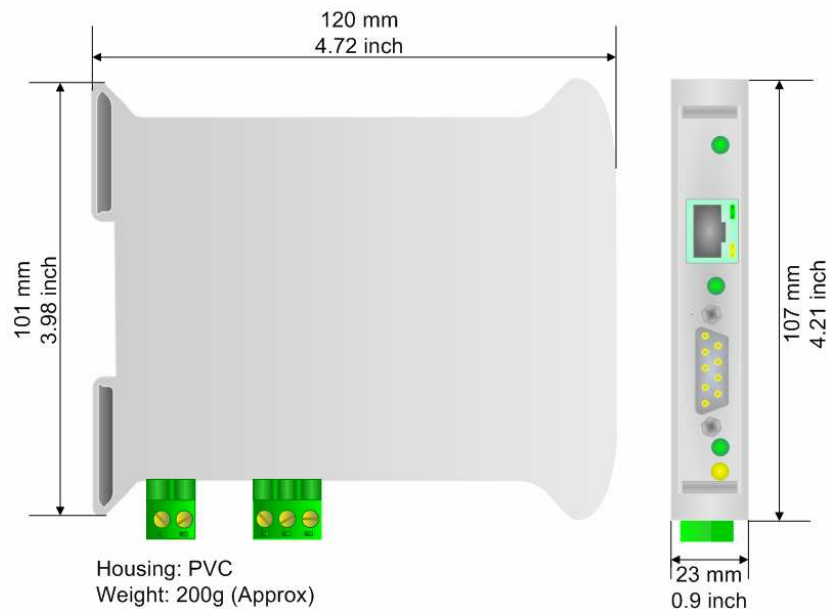
Figure 15: Mechanical dimensions scheme for HD67505
