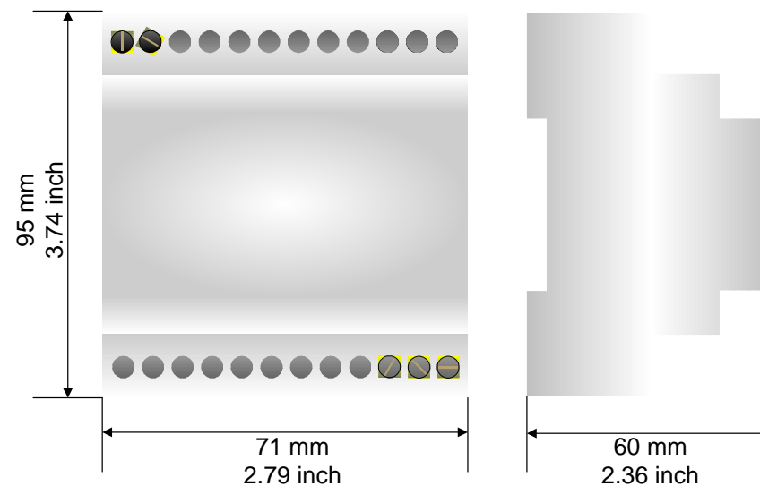
Figure 16: Mechanical dimensions scheme for HD67505M
