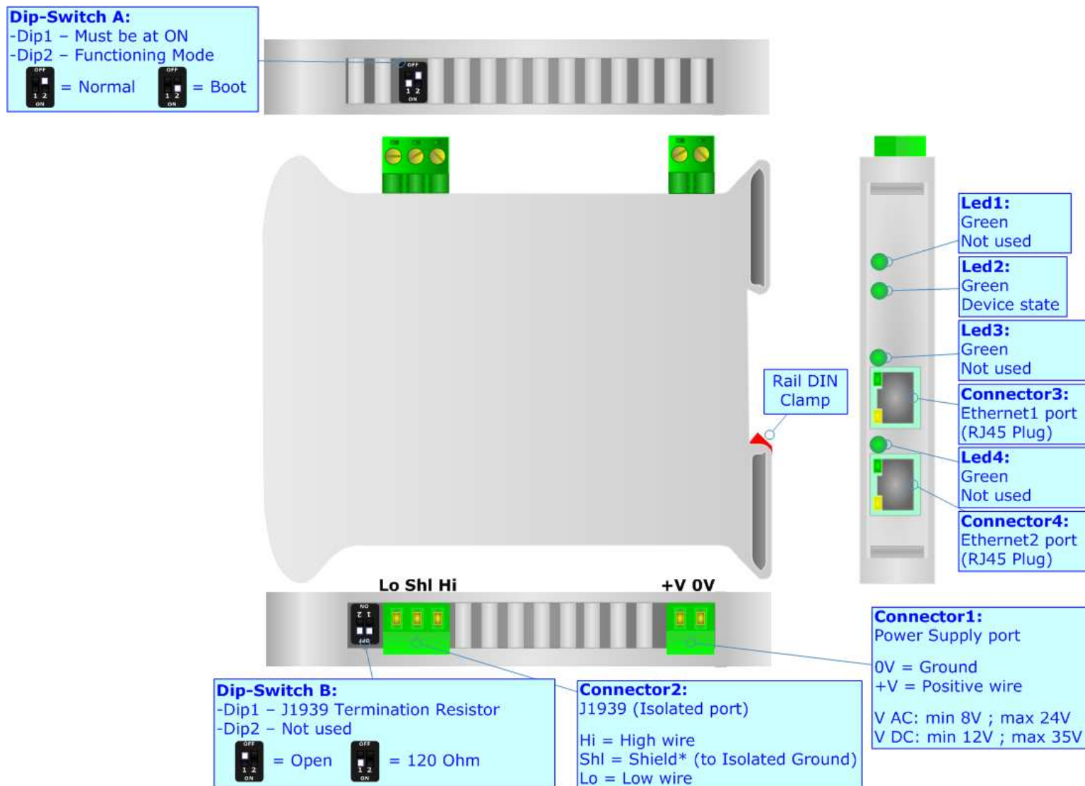
Figure 1: Connection scheme for HD67685-A1
