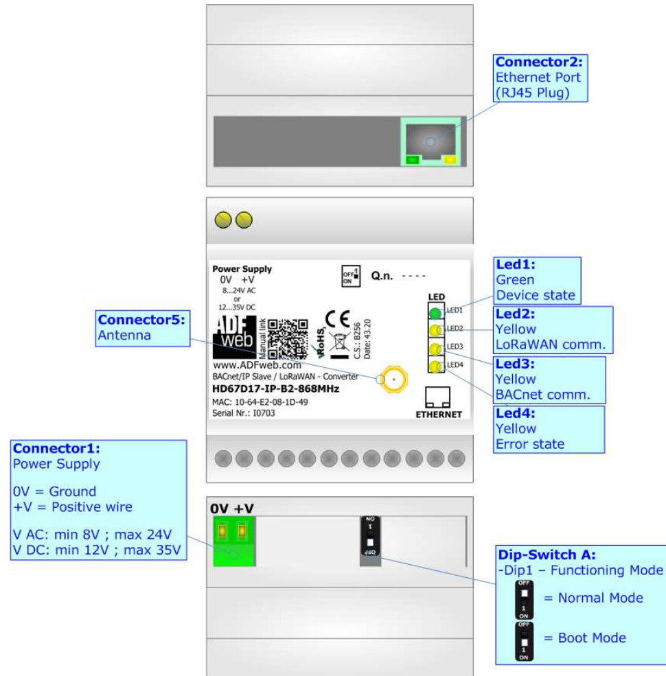
Figure 1a: Connection scheme for HD67D17-IP-B2-xxxMHz
