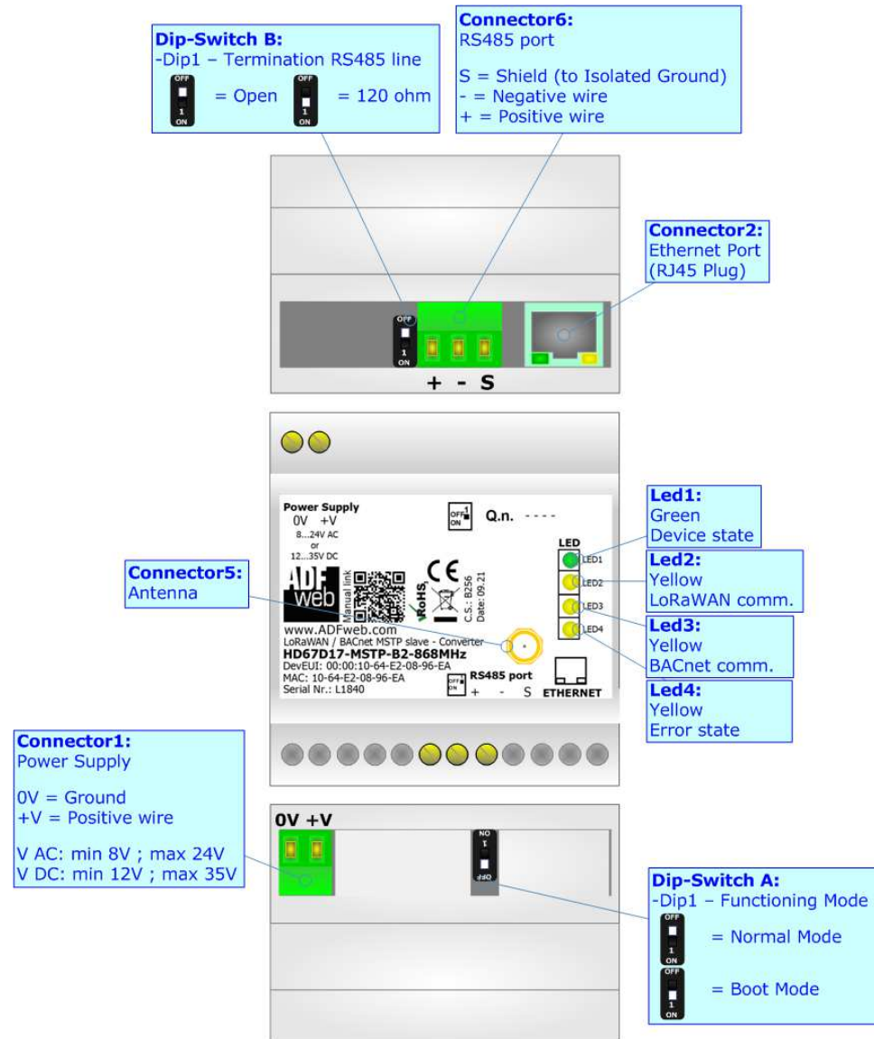
Figure 1b: Connection scheme for HD67D17-MSTP-B2-xxxMHz
