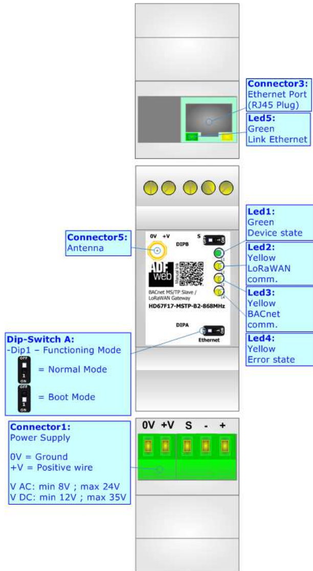
Figure 1b: Connection scheme for HD67F17-MSTP-B2-xxxMHz
