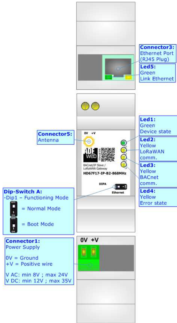
Figure 1a: Connection scheme for HD67F17-IP-B2-xxxMHz
