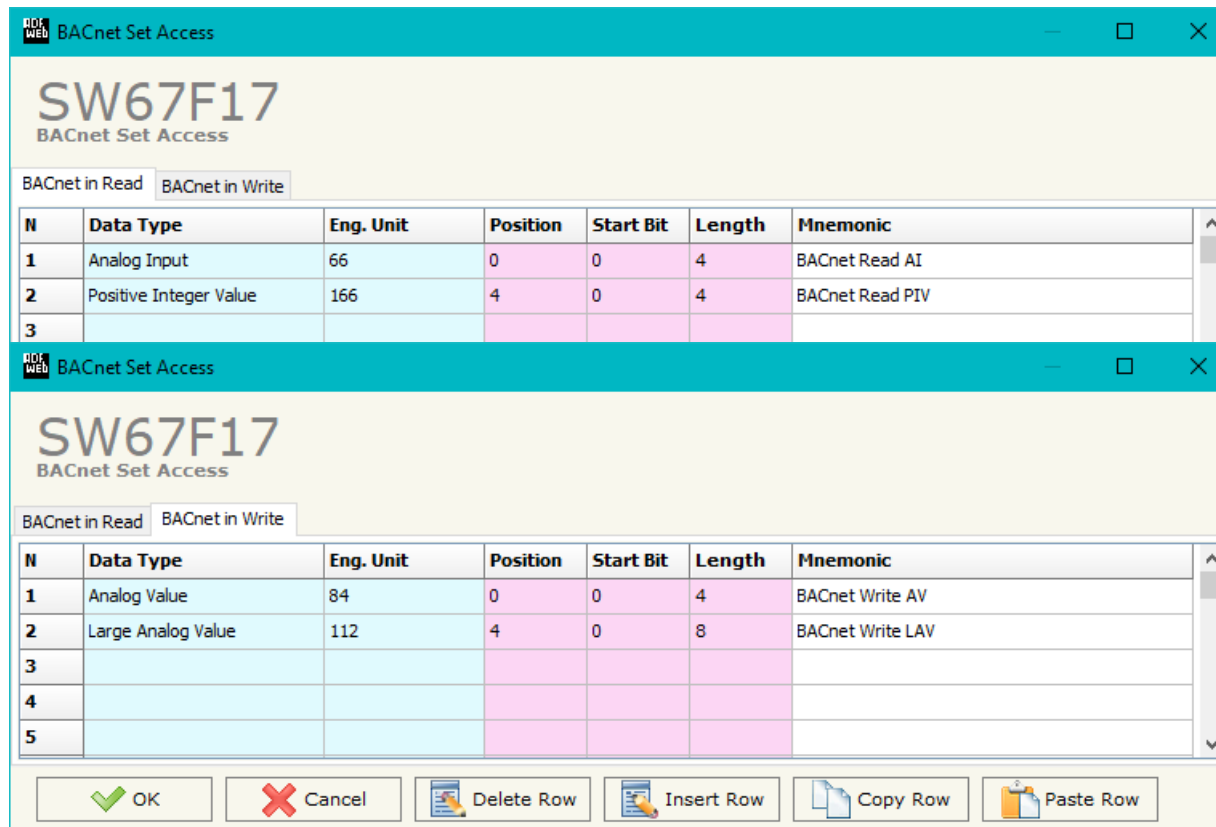
Figure 5: “BACnet Set Access” window
