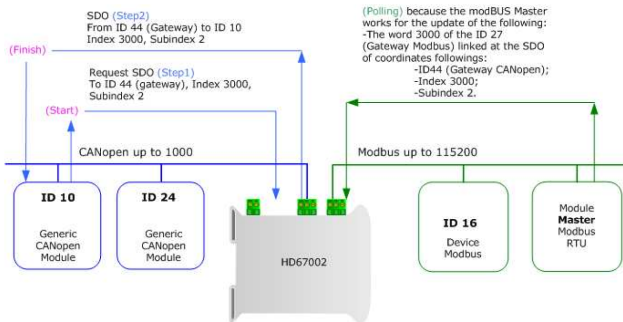
Figure 8: Chart of SDO request from Modbus side
