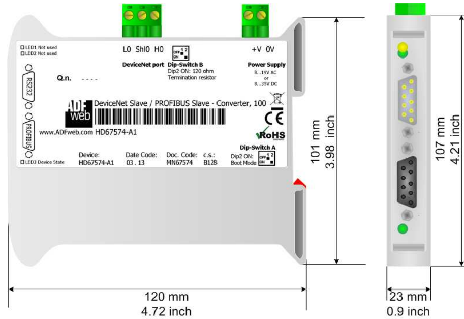
Figure 7: Mechanical dimensions scheme
