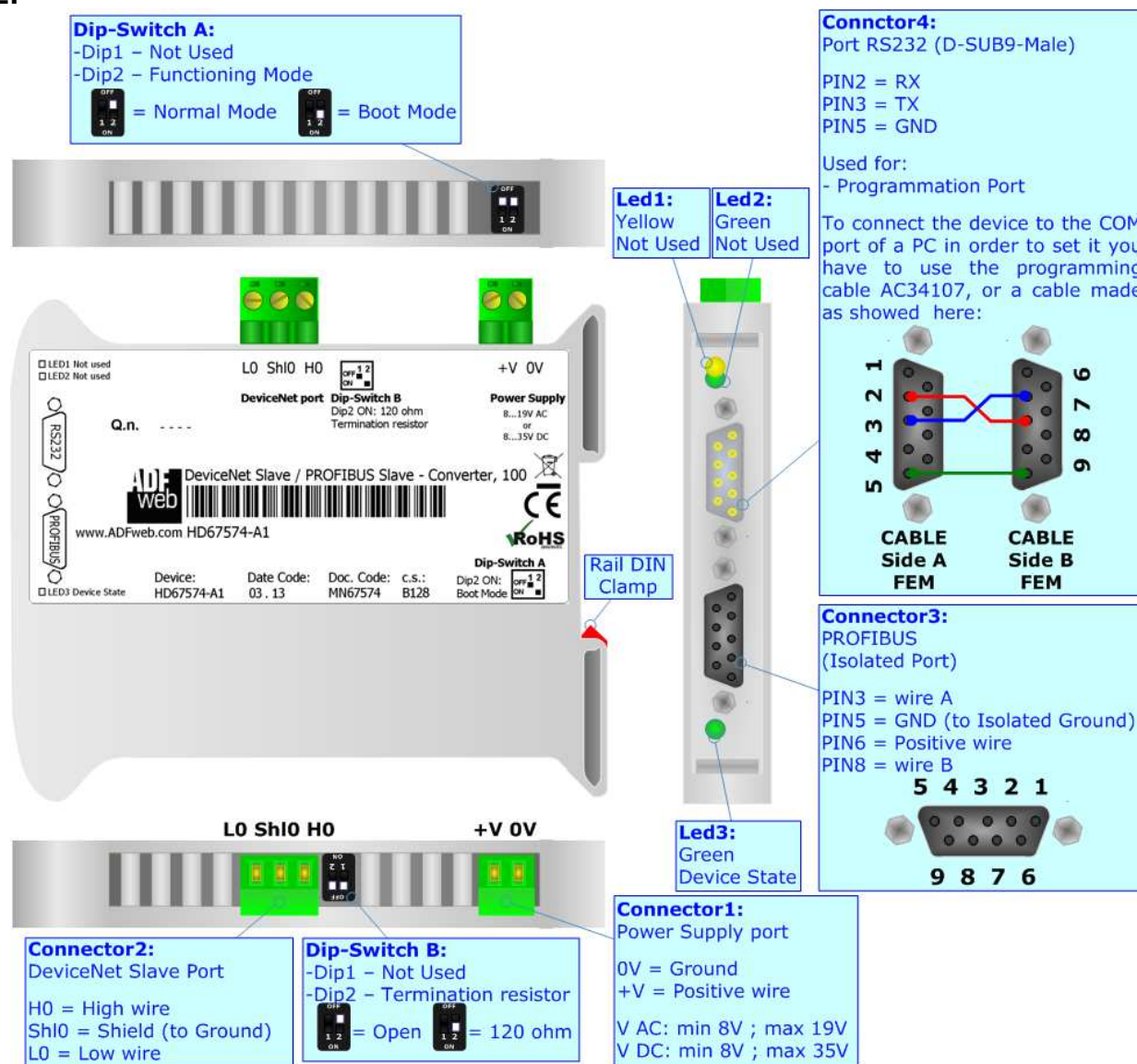
Figure 1: Connection scheme for HD67574-A1
