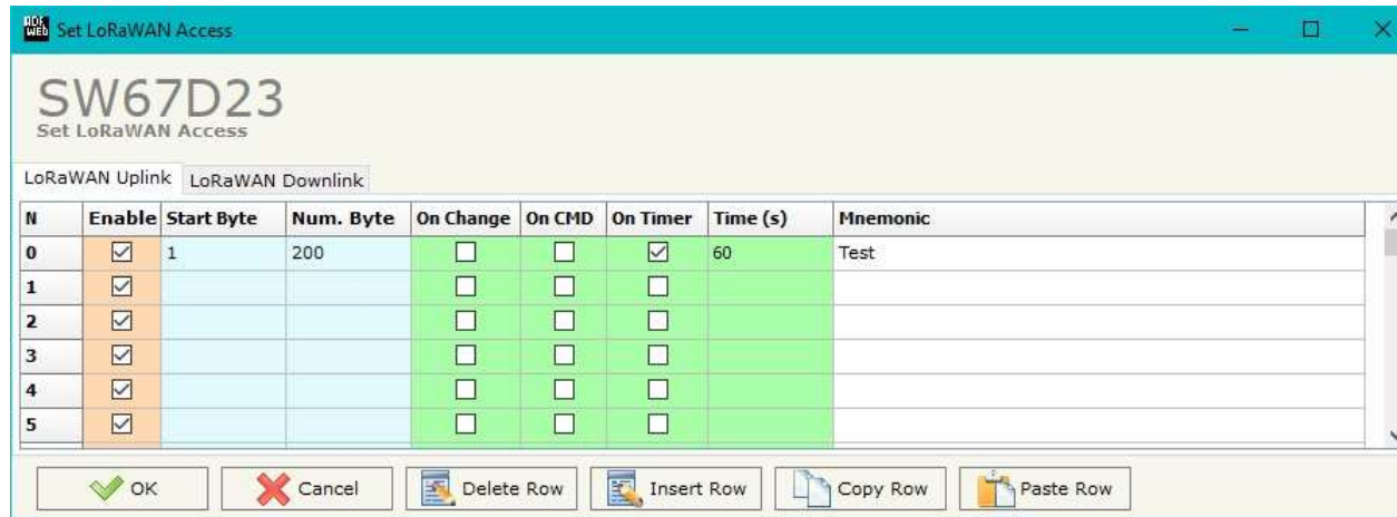
Figure 4a: “LoRAWAN Access → LoRaWAN Uplink” window
