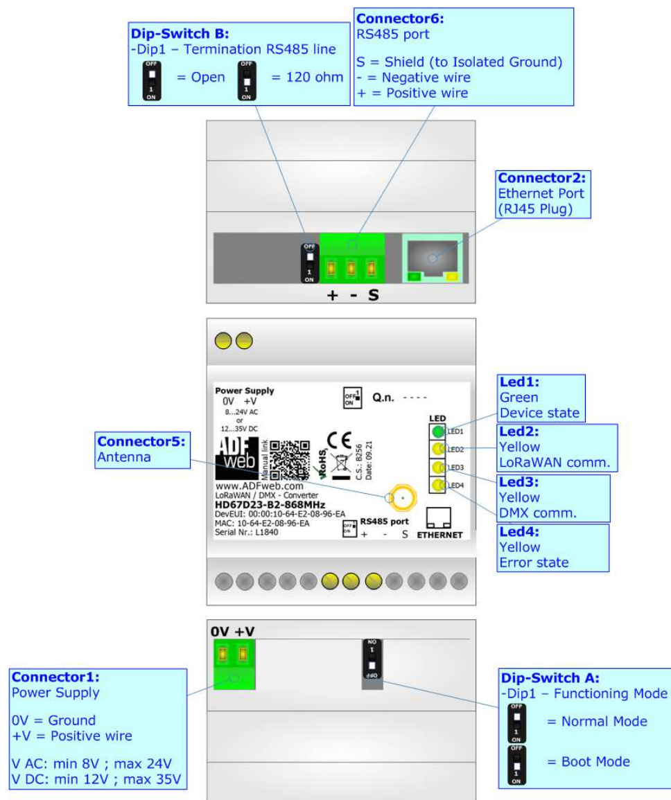
Figure 1: Connection scheme for HD67D23-B2-xxxMHz
