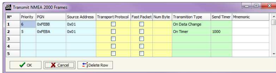
Figure 5: "Transmit NMEA 2000 Frames" window
