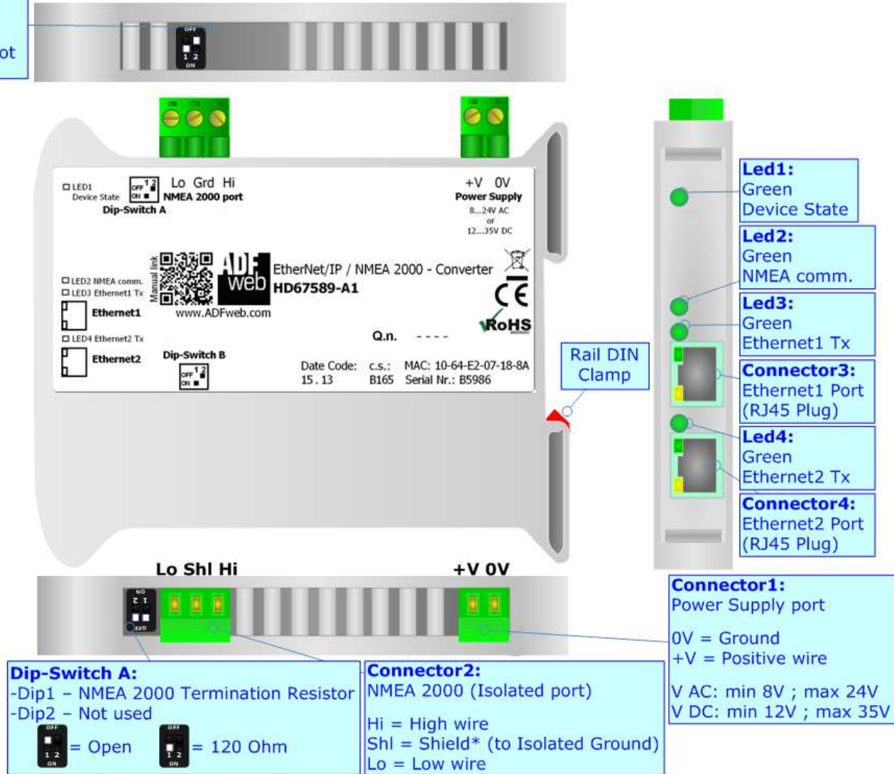
Figure 1: Connection scheme for HD67589-A1
