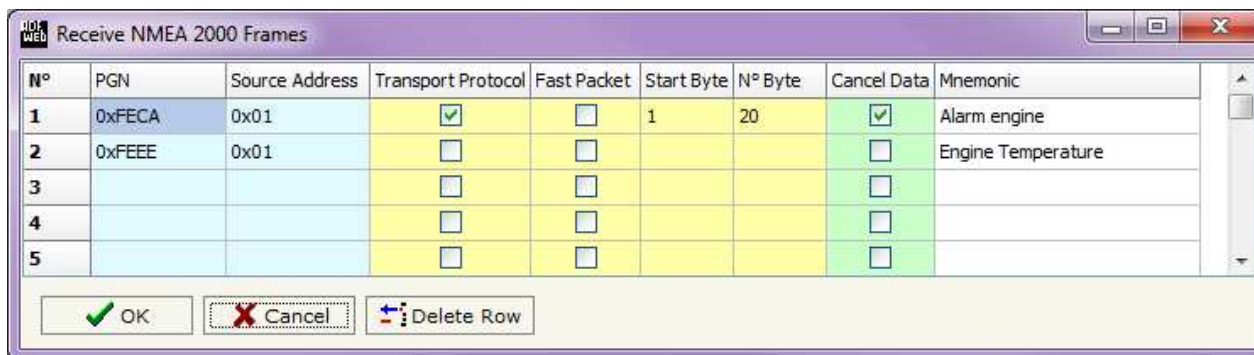
Figure 4: “Receive NMEA 2000 Frames” window
