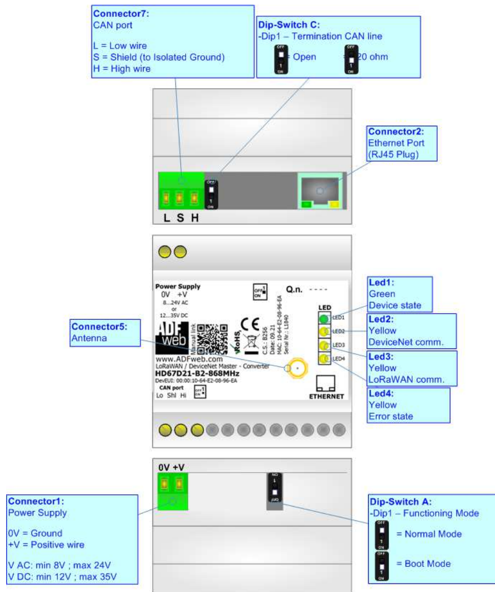
Figure 1: Connection scheme for HD67D21-B2-xxxMHz
