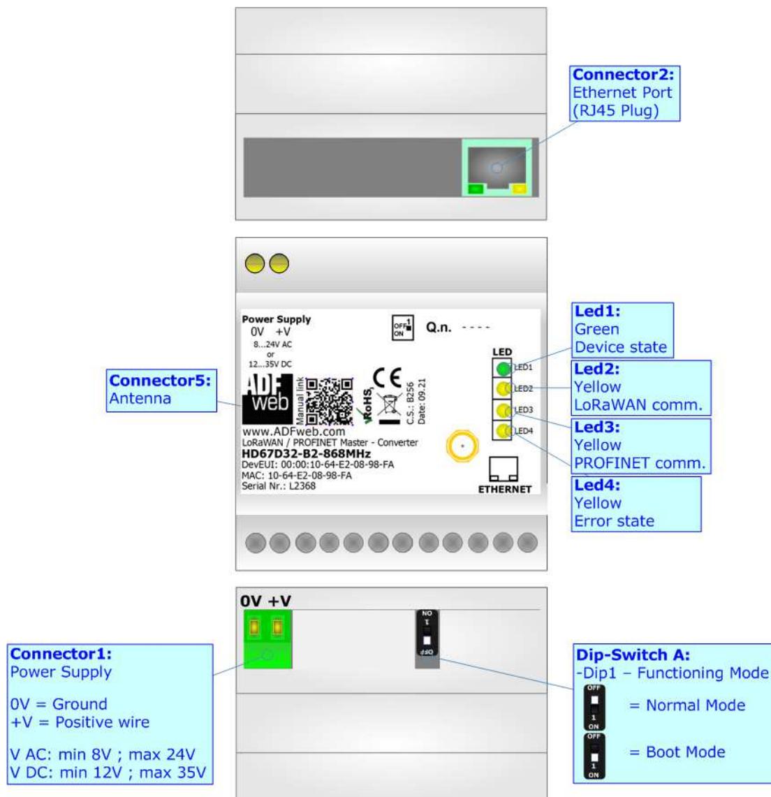
Figure 1: Connection scheme for HD67D32-B2-xxxMHz
