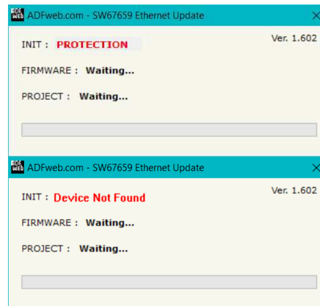
Figure 5: Error windows
