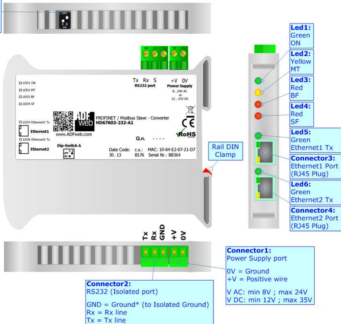
Figure 1a: Connection scheme for HD67603-232-A1
