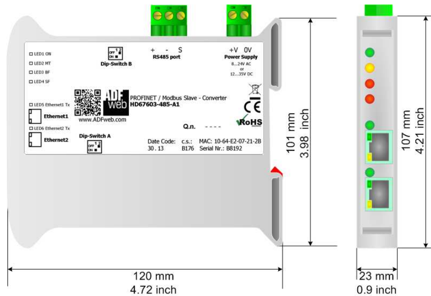
Figure 6b: Mechanical dimensions scheme for HD67603-485-A1
