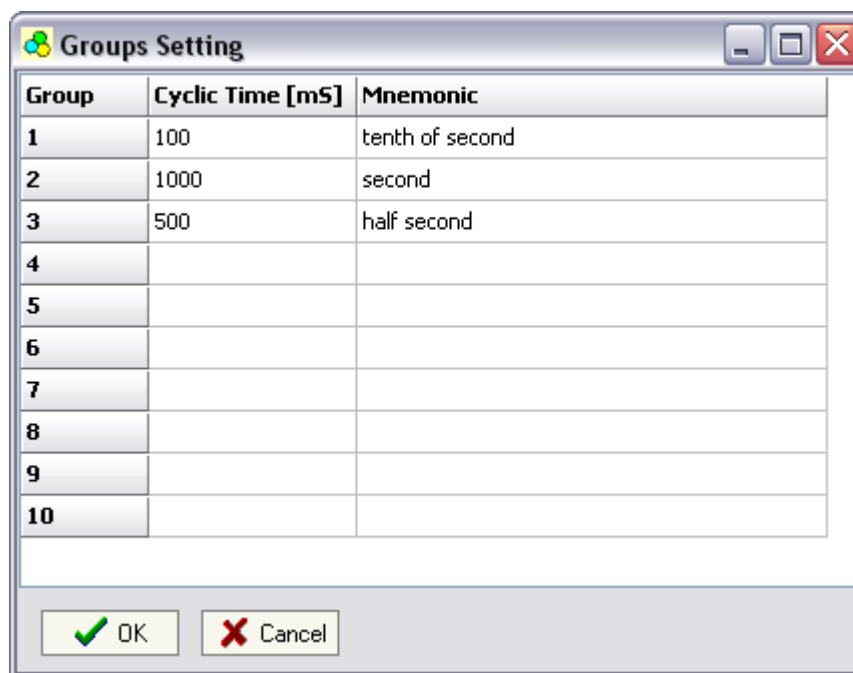
Figure 7: "Groups Setting" window
