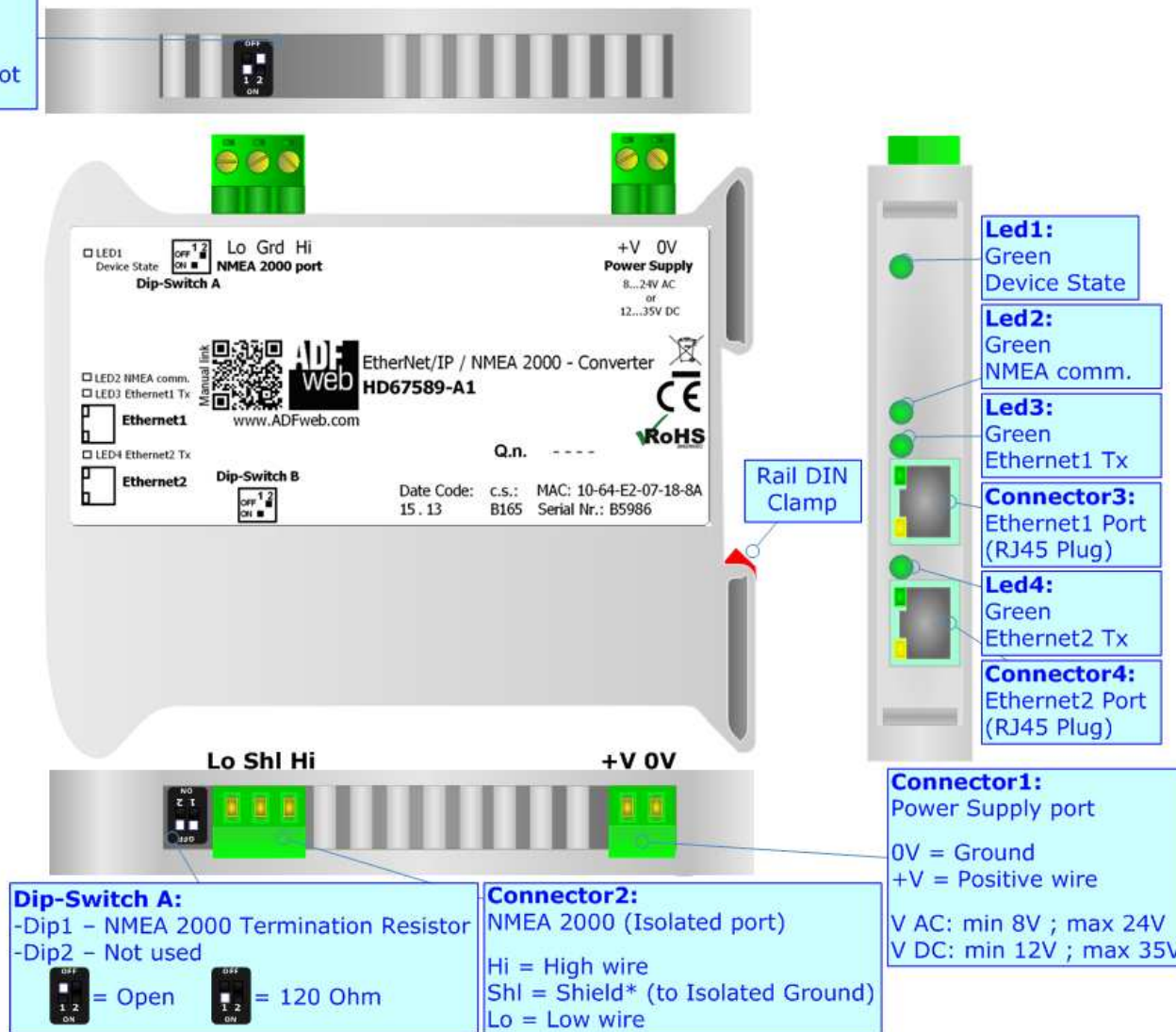
Figure 1: Connection scheme for HD67589-A1
